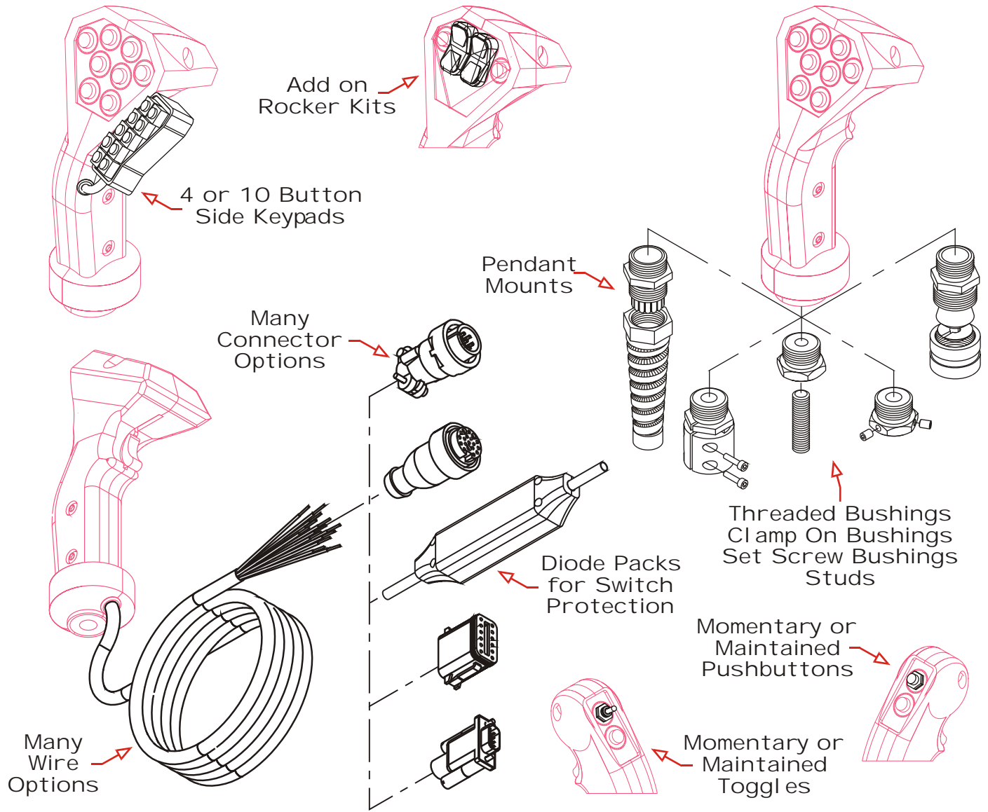
"JS" Series Joystick
