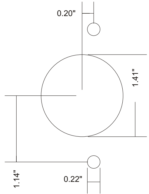
Panel Mounting Dimensions
